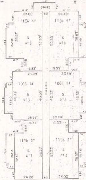
TYPE 3 BUILDING FIRST FLOOR PLAN
