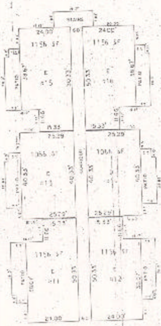
TYPE 3 BUILDING FIRST FLOOR PLAN
