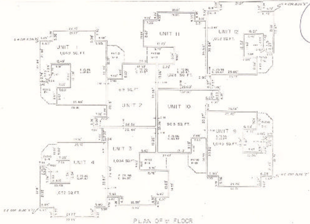
PLAN OF 1st FLOOR BUILDING E
